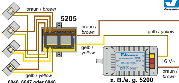
Tip: viessmann item 5205 Power module with distribution strip Avoids flickering with AC power supply. Nearly double brightness of the lamps.
